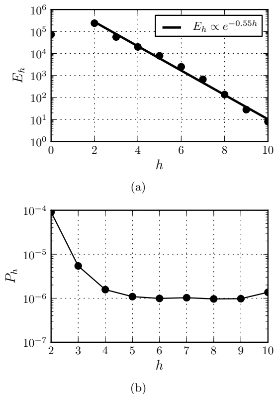
Figure 5: Number of new links E_h created between nodes h hops away (a) and probability P_h that a new link connects nodes h hops away. The single E_h value at h = 0 denotes the number of edges connecting nodes previously in separate disconnected components.
