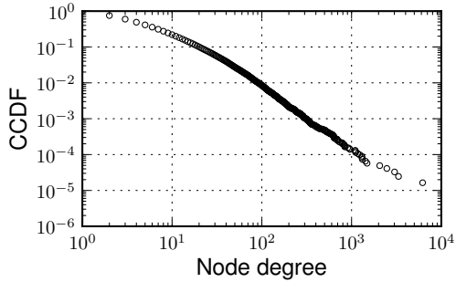
(a) Node degree
